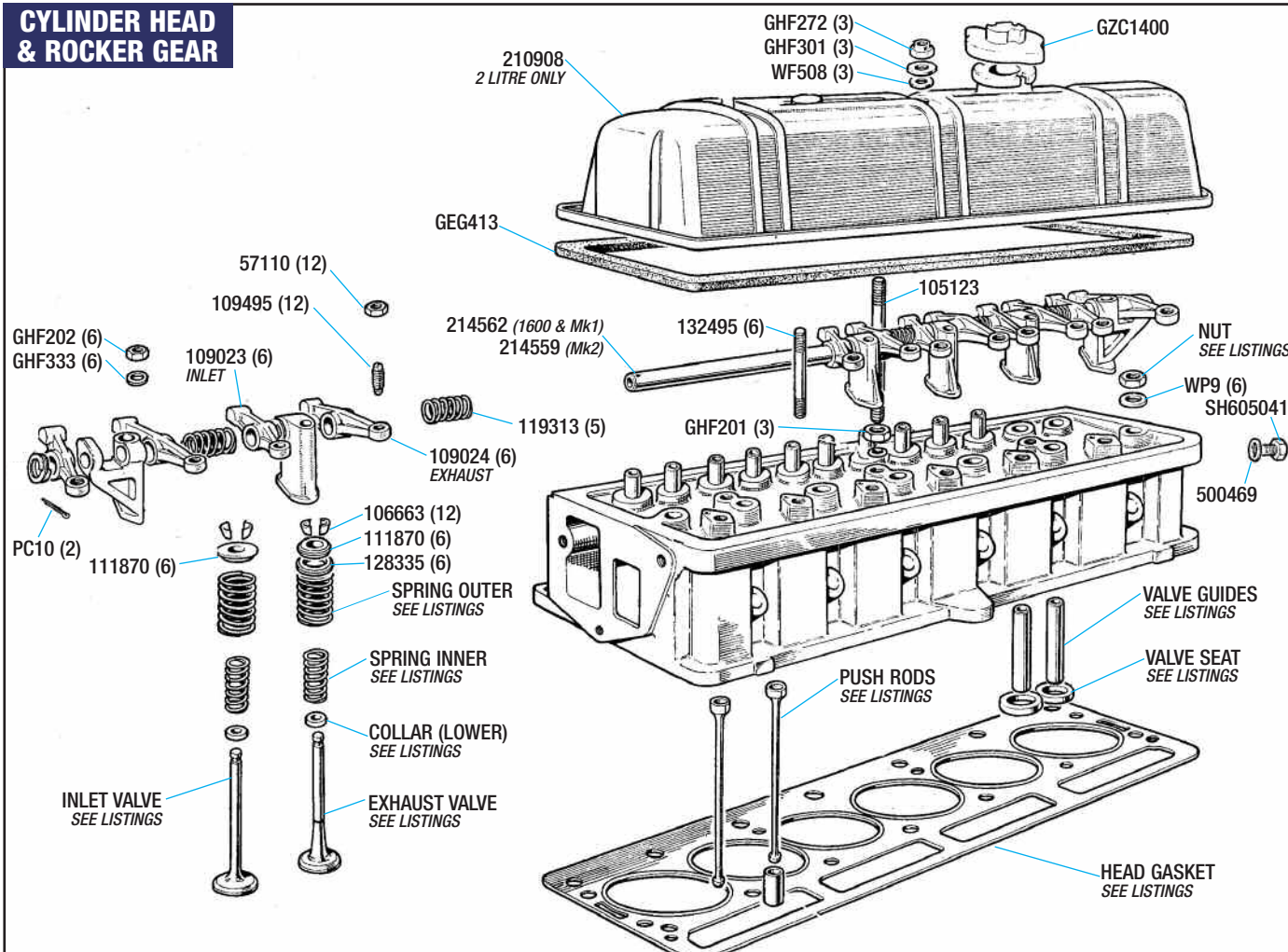
CYLINDER HEAD REBUILD KIT (MK2 2 LITRE) RV6005RBK
