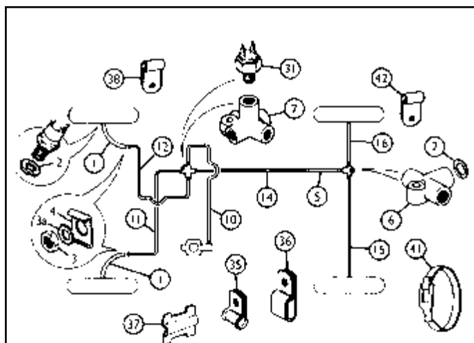
Single Line System, 1962 - '67
