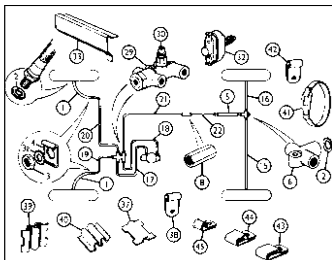
Dual Line, Non-Servo, 1968 - '74
