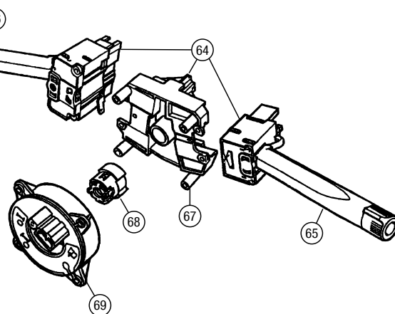
IGNITION SWITCH/ STEERING LOCK - RHD - QRF101080
