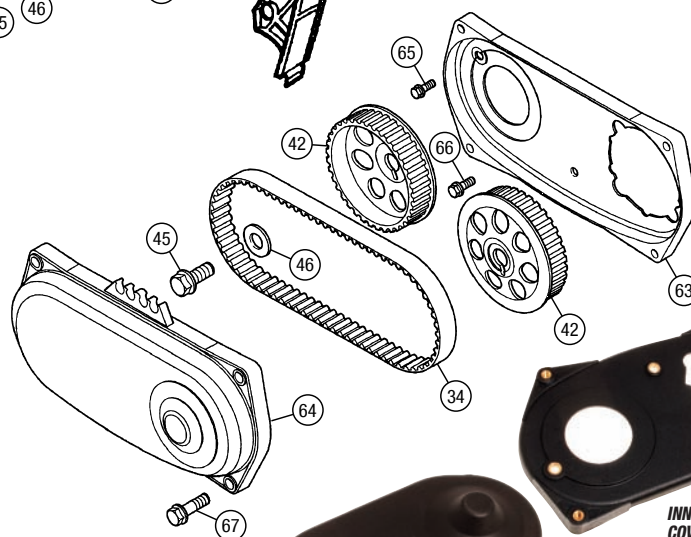
OUTER REAR TIMING COVER - MG TF VVC TYPE - LJR000120
